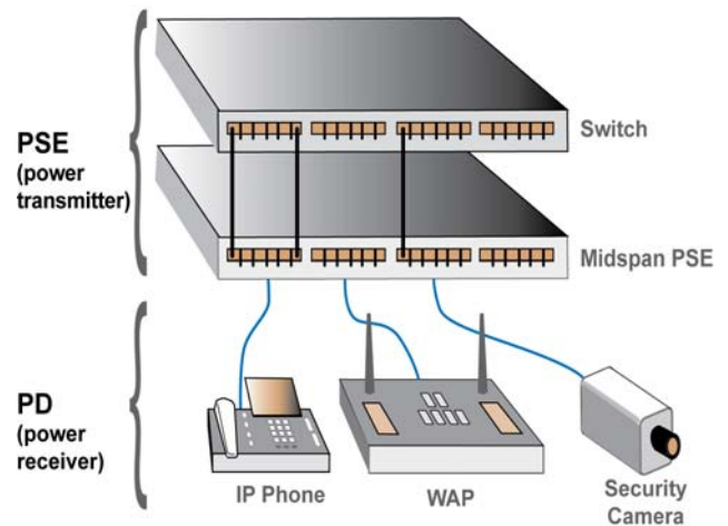
Figure 1: Typical PoE System Arrangement
