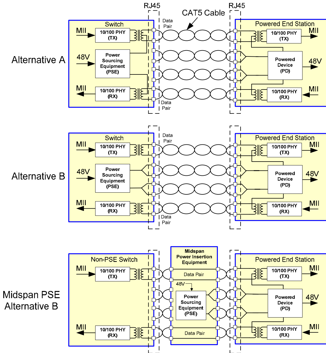
Figure 3: 10/100 Power Feed Alternatives
