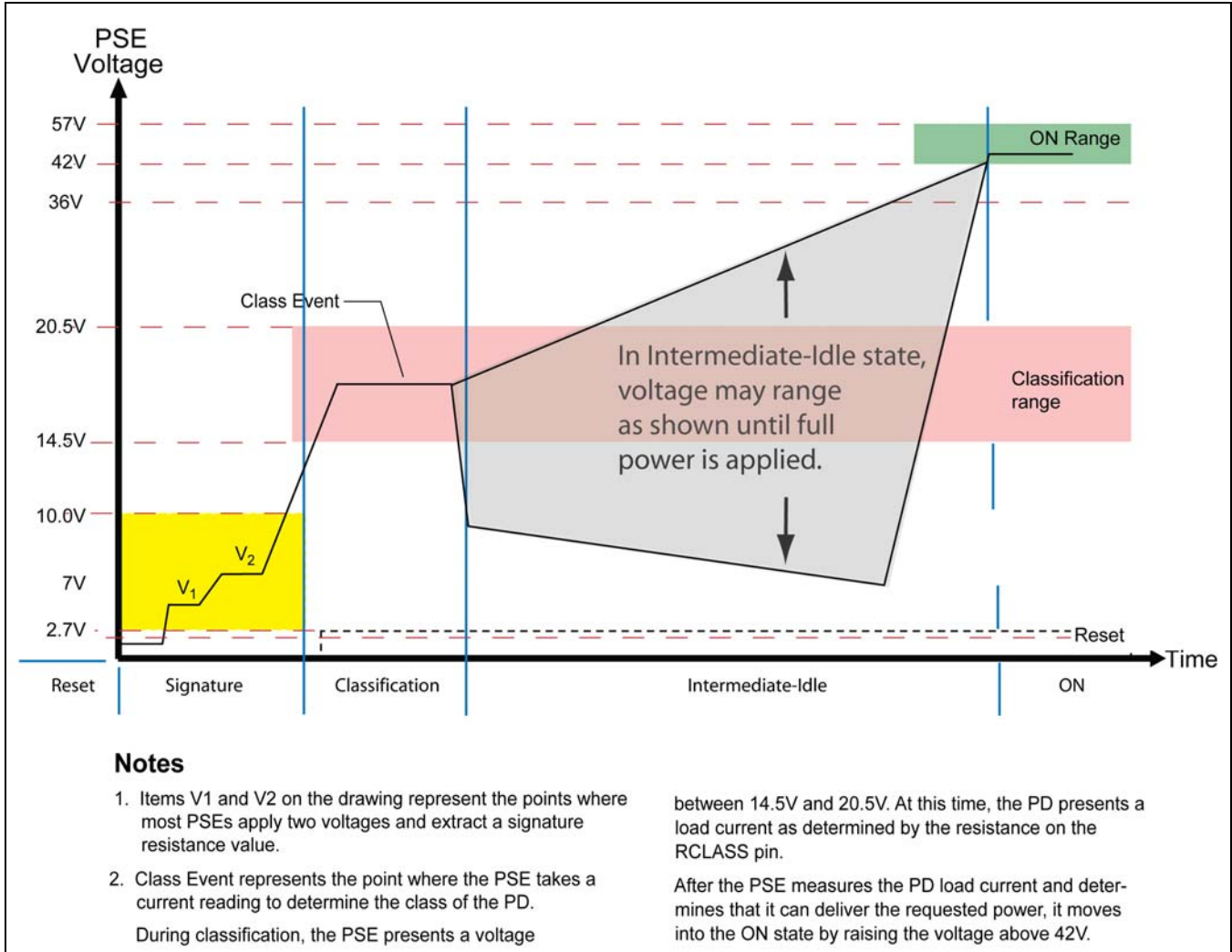
Figure 2: PoE Waveform
