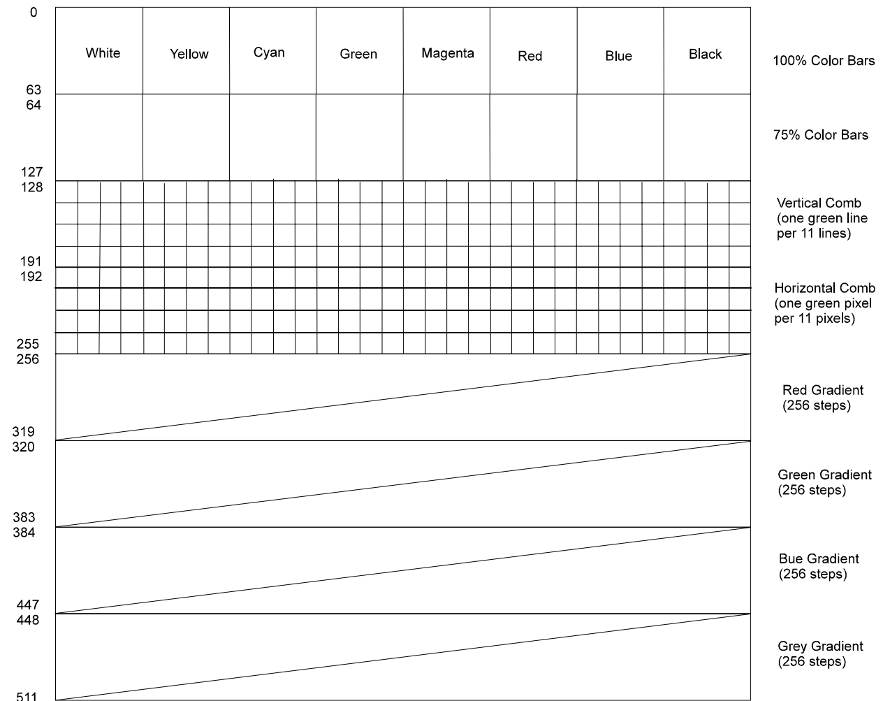
Figure 7: BiPGEN Image
